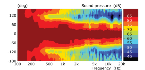
Reference 5 Meta Spinorama (top) and dispersion plots - horizontal (middle) and vertical (bottom)
