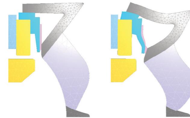
Figure 5. FEA simulation of exaggerated deformation of tangerine waveguide and surround support at 12kHz
