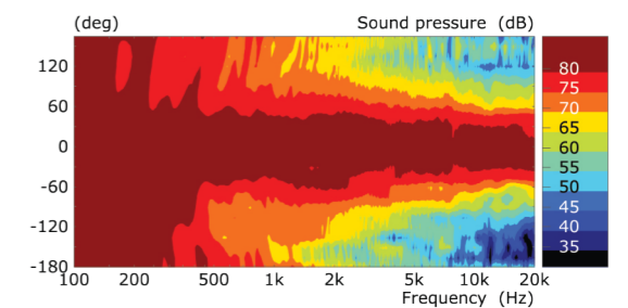
Reference 1 Meta Spinorama (top) and dispersion plots - horizontal (middle) and vertical (bottom)
